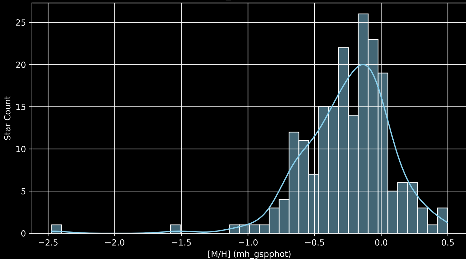
APOGEE DR17 Field: [055-53-O] [M/H] (mh_gspphot) (n= 201)
