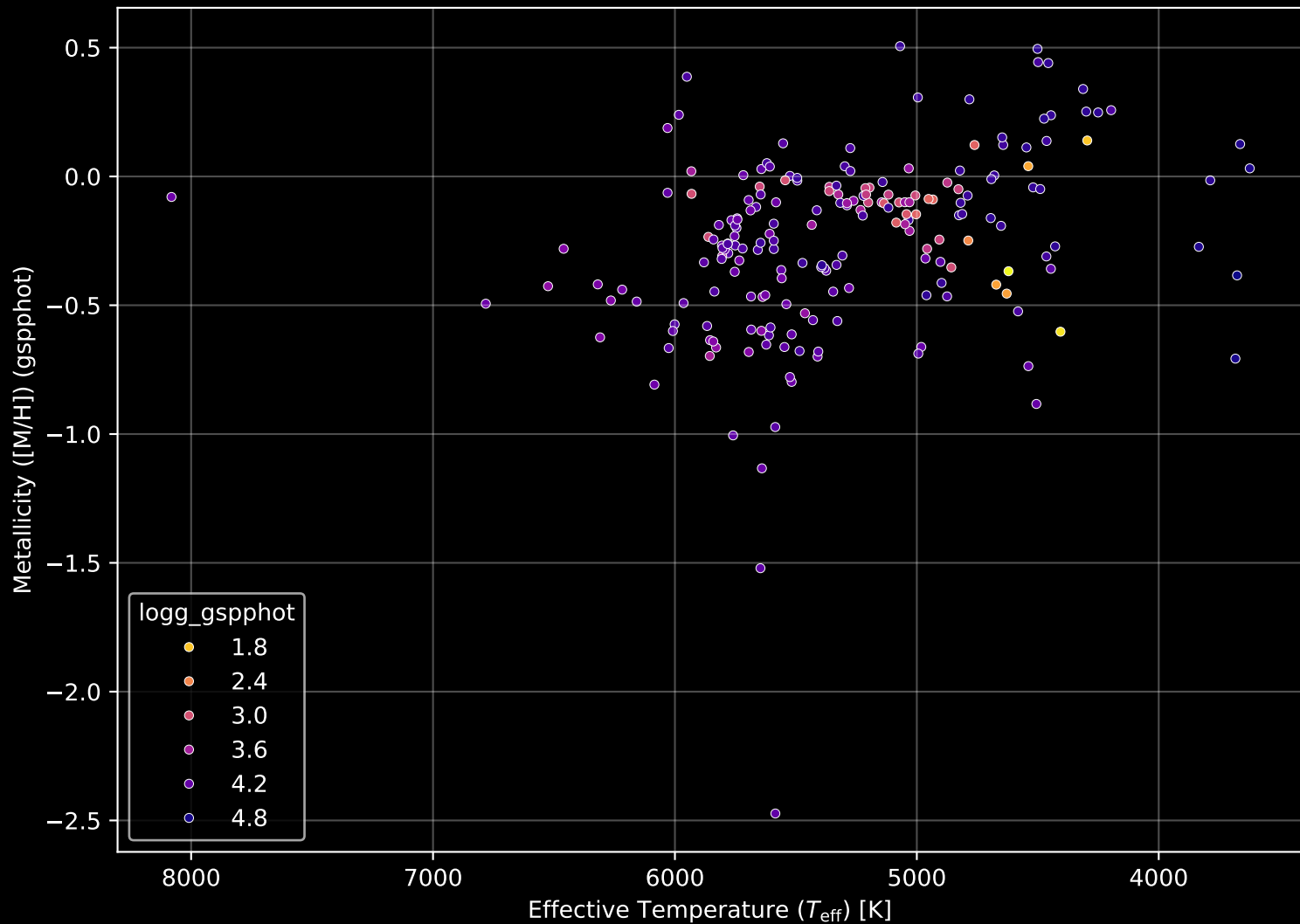
APOGEE DR17 Field: [055-53-O] Stellar Population Parameters (n= 202)
