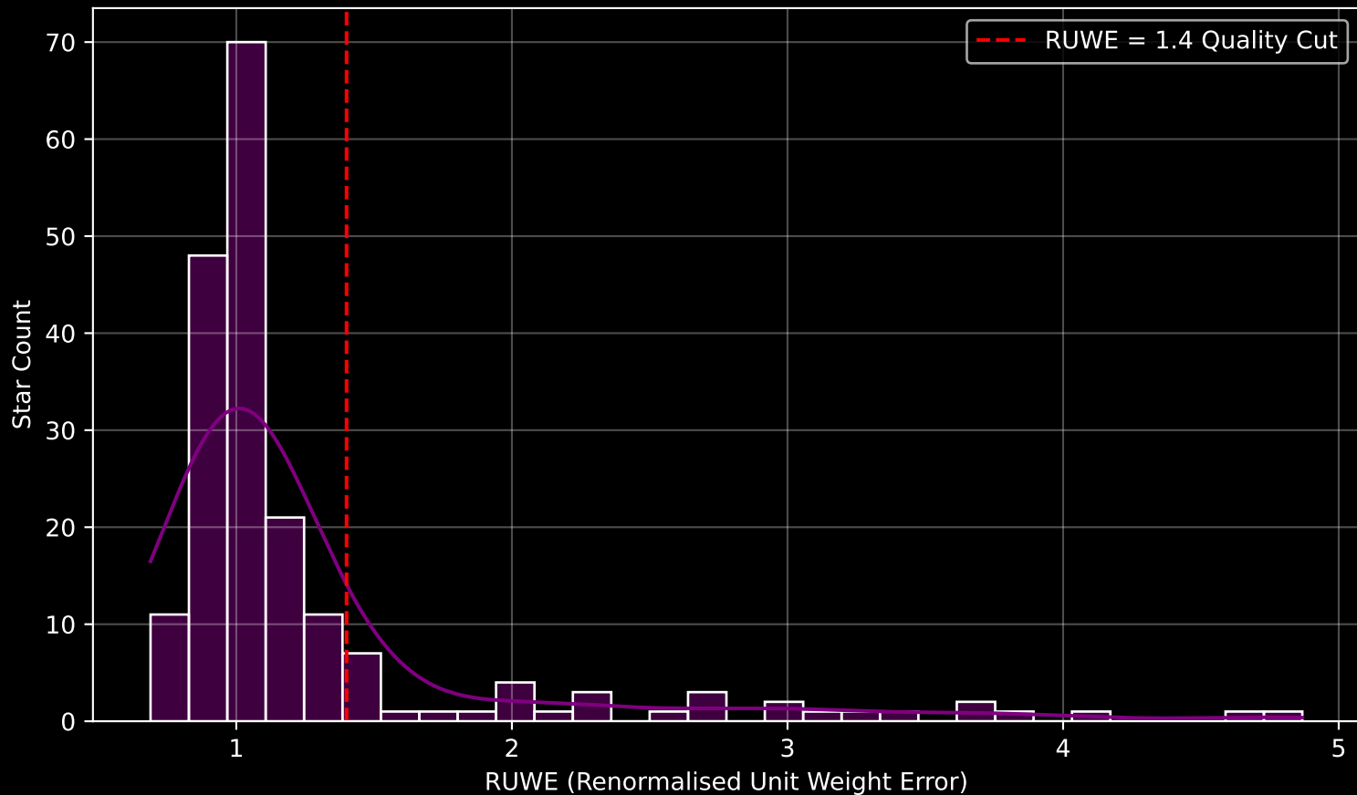
GAPOGEE DR17 Field [055-53-O] RUWE Distribution (n= 194)
