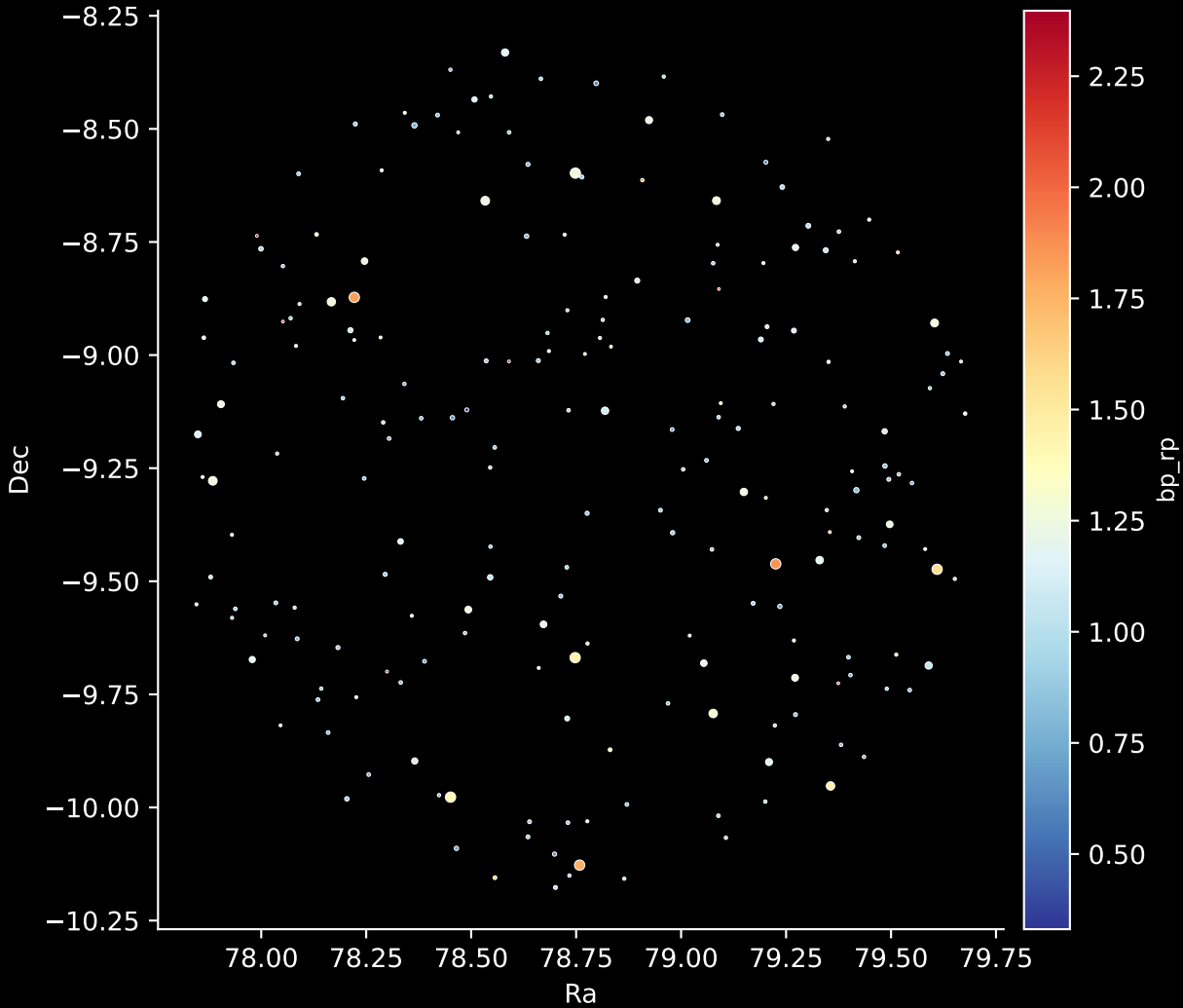
APOGEE DR17 Field: [055-53-O] Stars: 202
