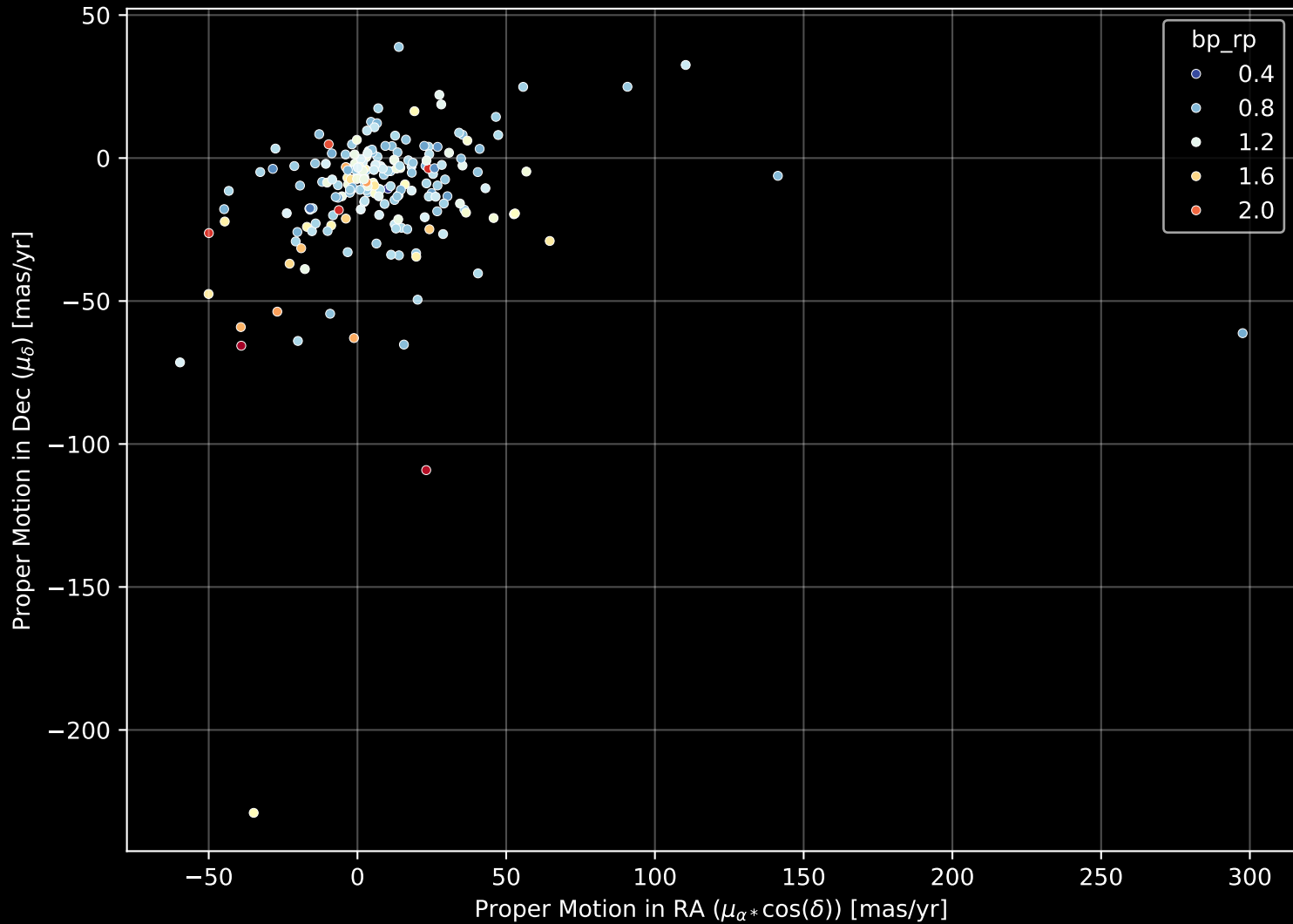
APOGEE DR17 Field: [055-53-O] Proper Motion Diagram (n= 202)
