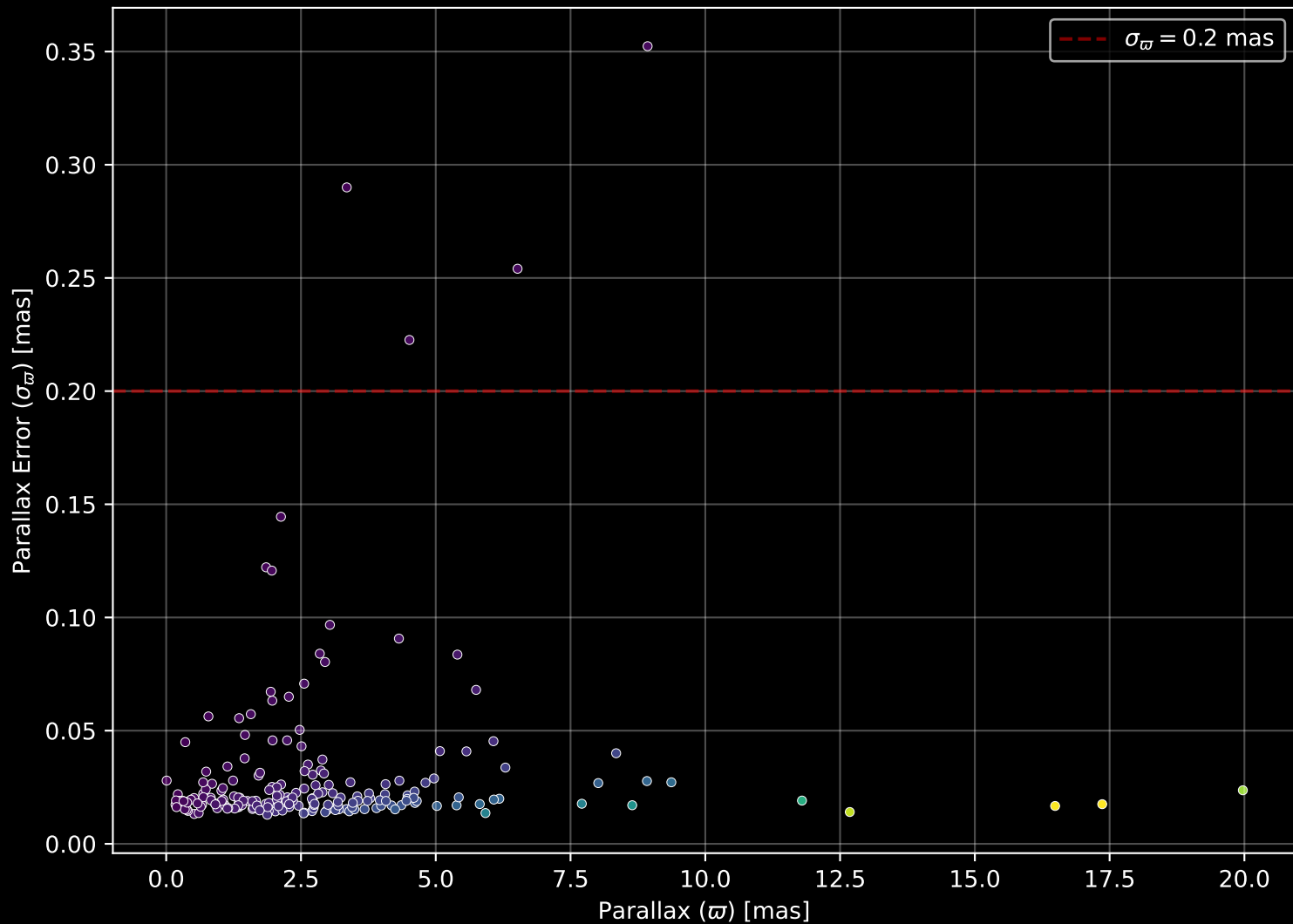
APOGEE DR17 Field: [055-53-O] Parallax Quality (n= 202)
