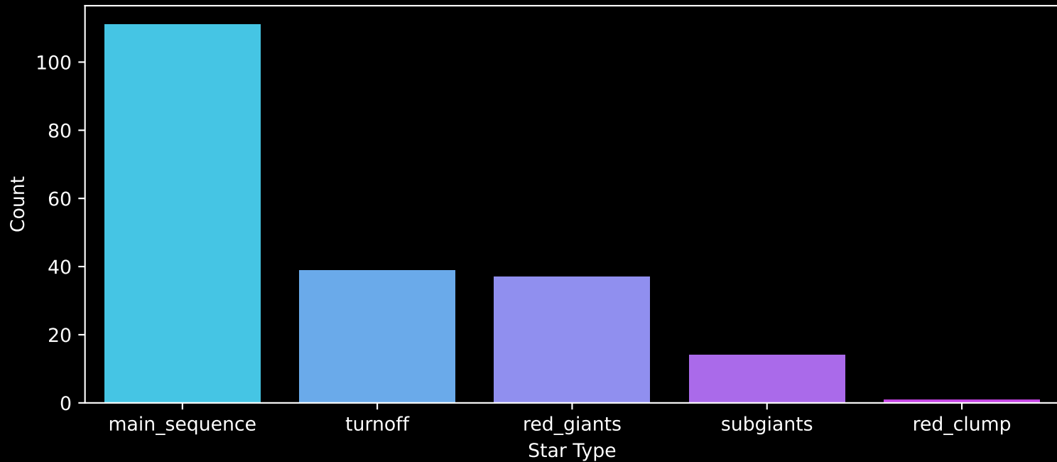
APOGEE DR17 Field: [055-53-O] Count plot of Star Type
